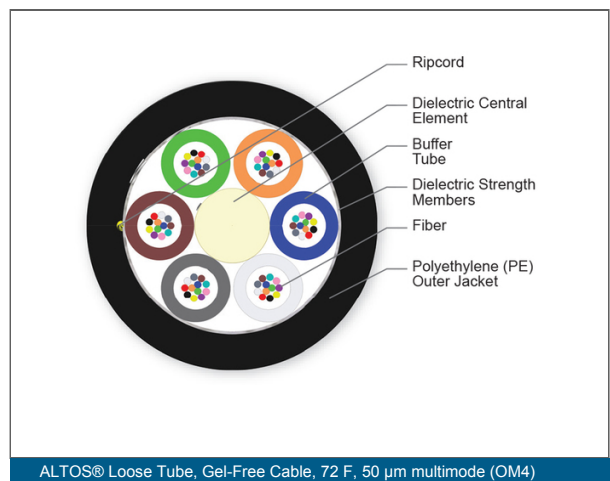
ALTOS® Loose Tube, Gel-Free Cable, 72 F, 50 µm multimode (OM4)
